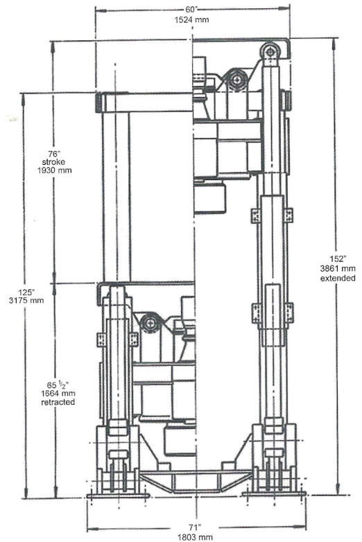
derrick position
